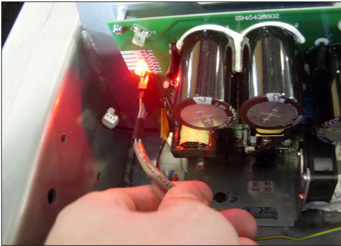
2 of the 3 console cable connections at the motor tray (the other is the coax cable).
