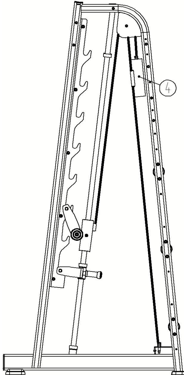
Wire rope alignment diagram
