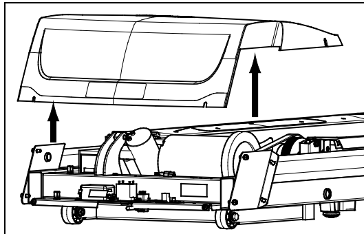
Figure 6: Hood removal
