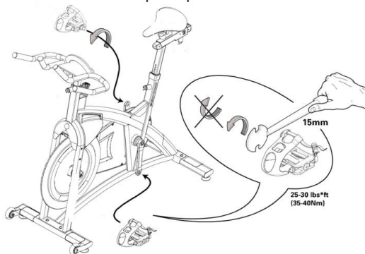
Example of pedal installation
